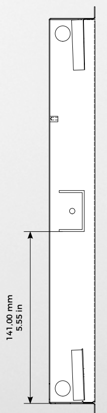
Flush-mounting housing (backbox)
