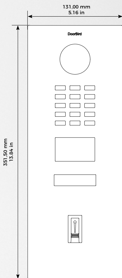
Front panel
