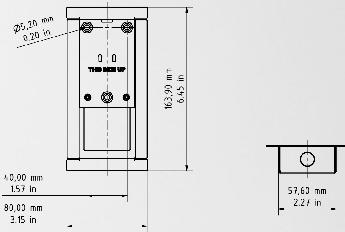
D1101V Flush-mounting housing (backbox)
