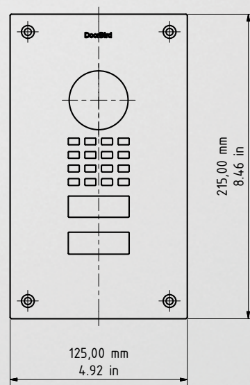
Front panel
